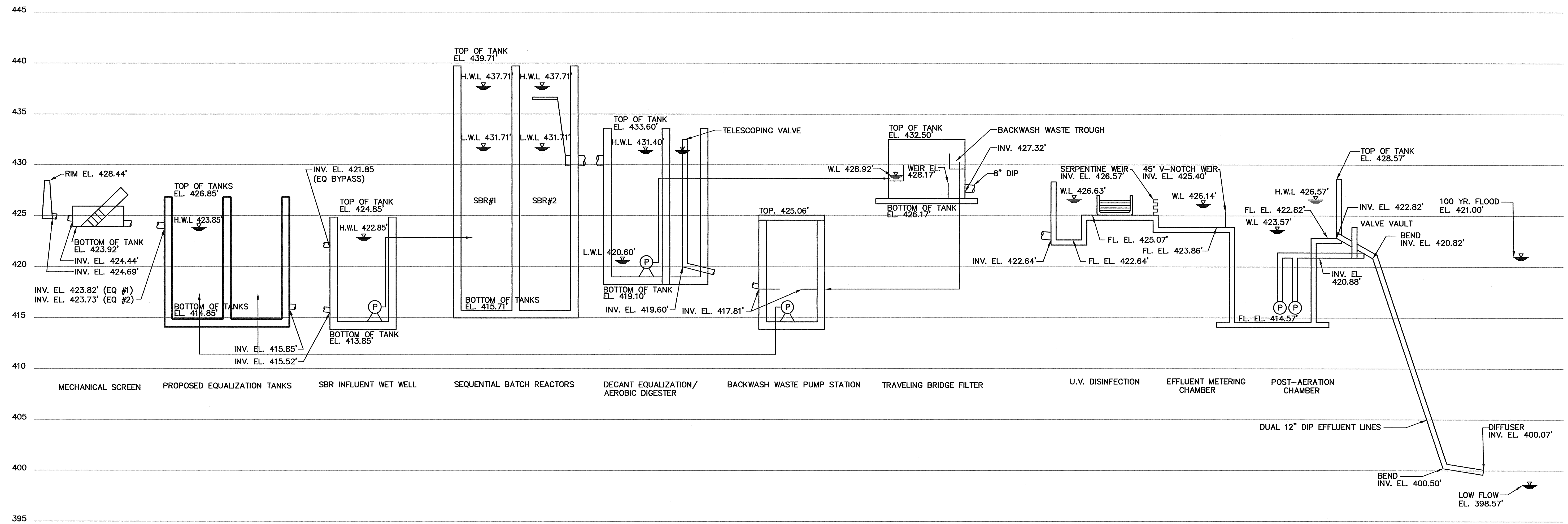
HYDRAULIC PROFILE HORIZONTAL SCALE: NONE VERTICAL SCALE: 1" = 5'
